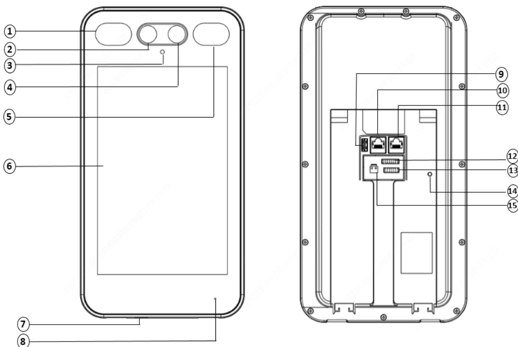
Figure3-1 Device Structure
